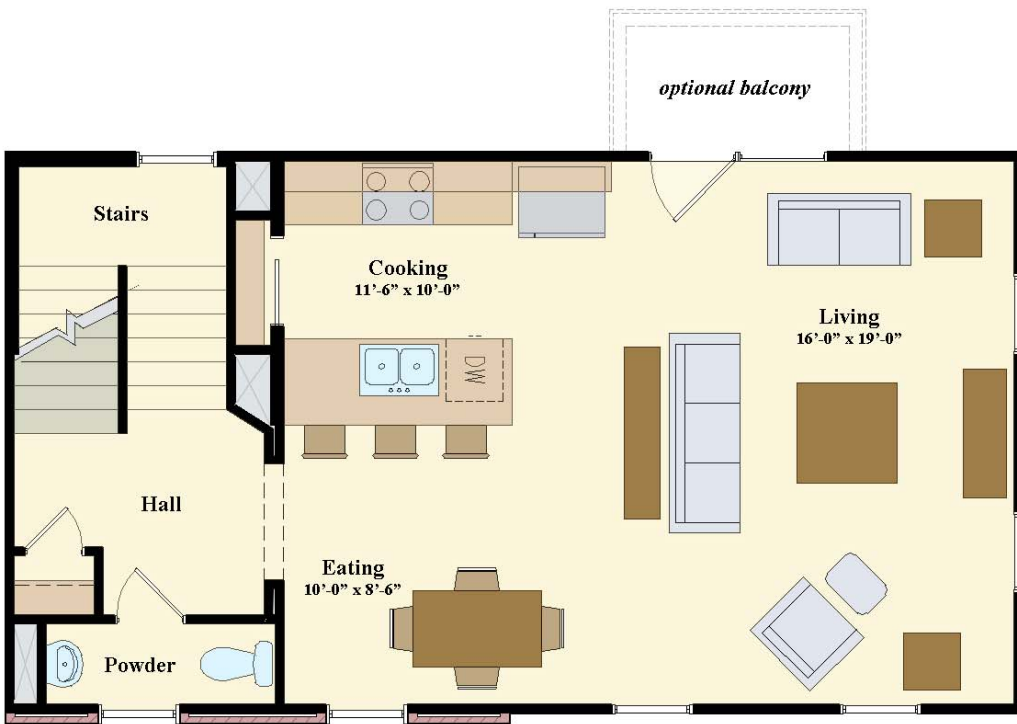
Unit A Main Level Floor Plan
