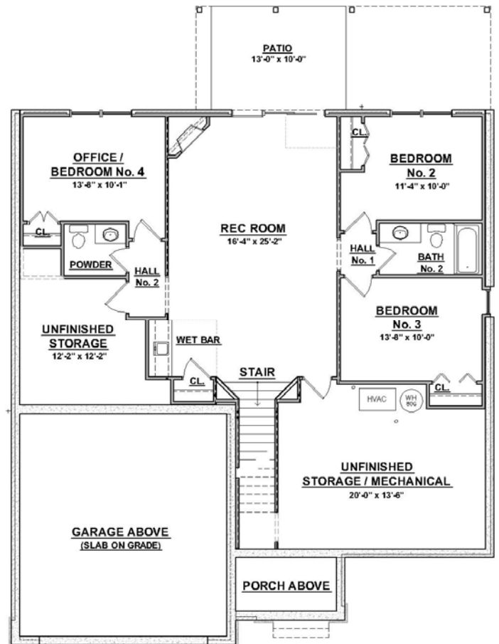
Lower Level Floor Plan 1126 finished square feet
