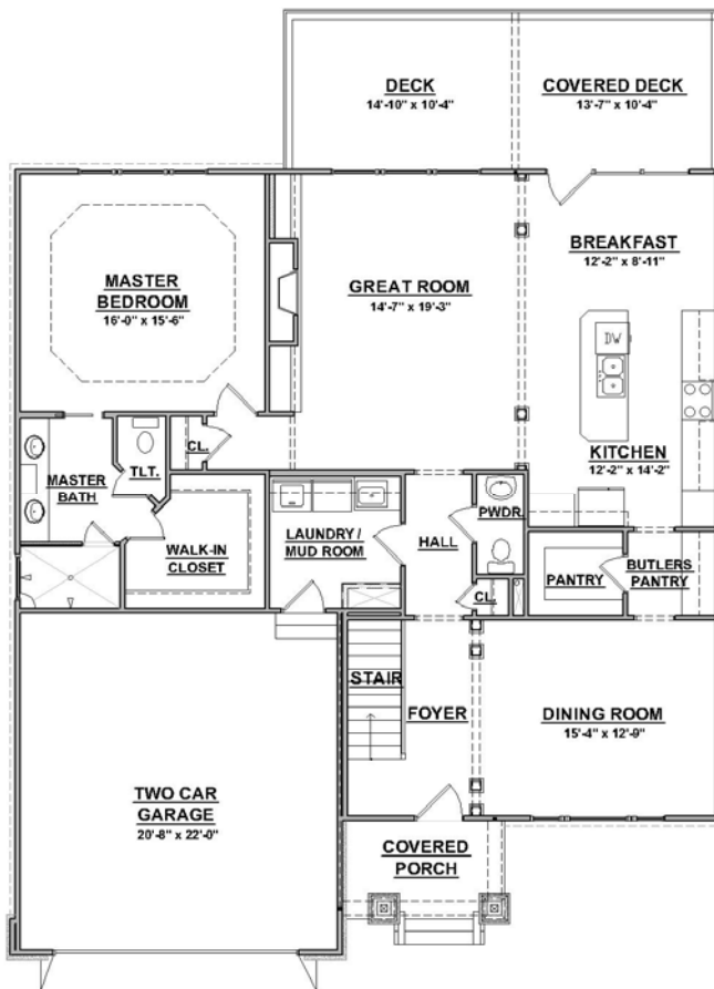
Main Level Floor Plan 1674 finished square feet
