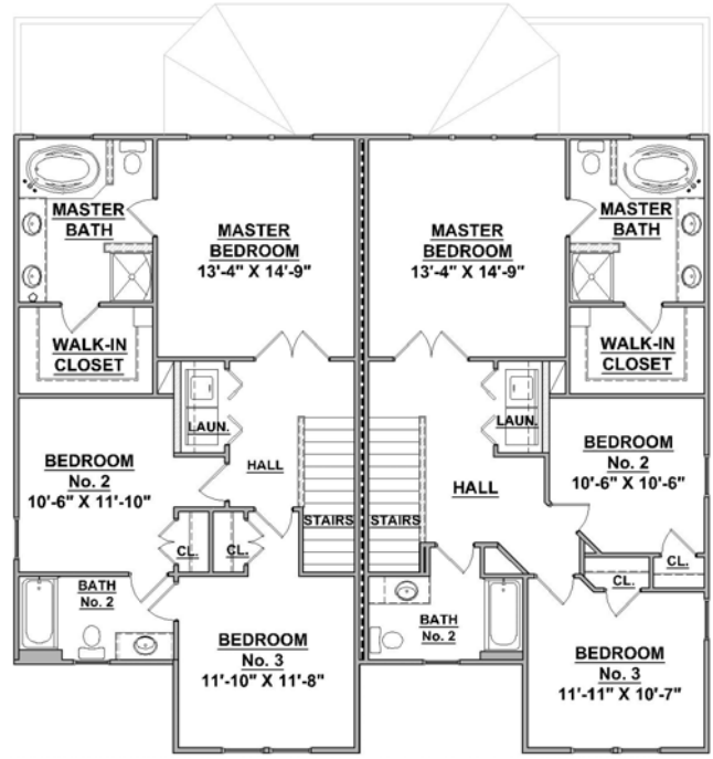
Upper Level Floor Plan 917 square feet
