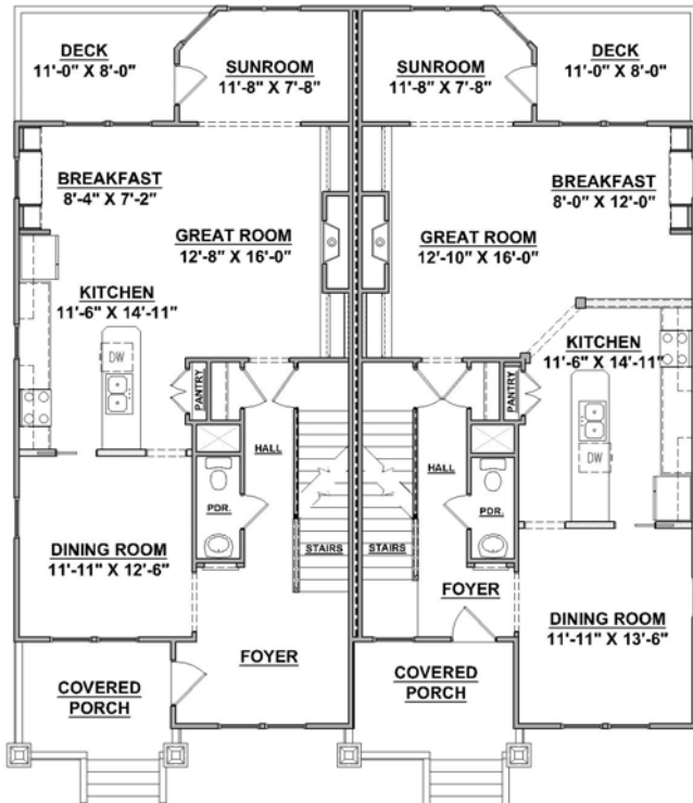
Main Level Floor Plan 1011 square feet
